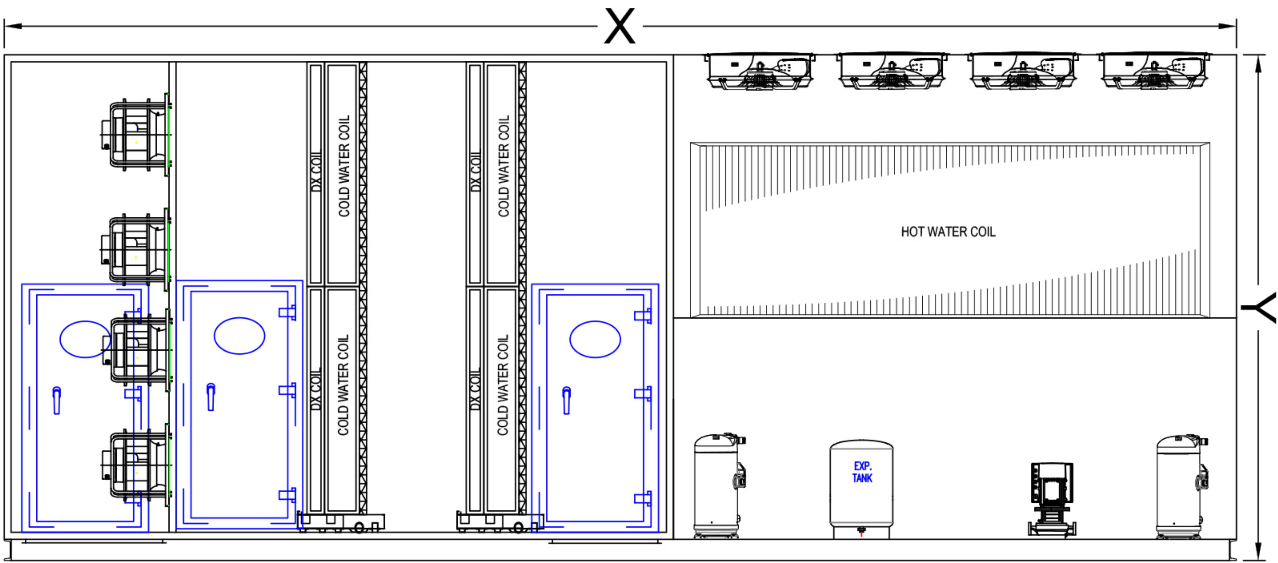
FRONT VIEW
