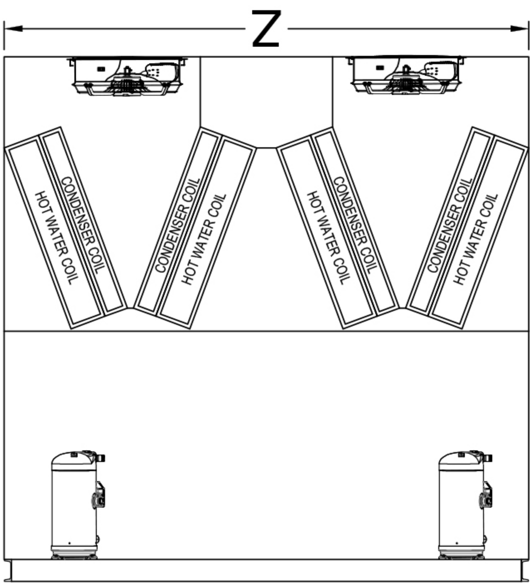
SIDE VIEW
